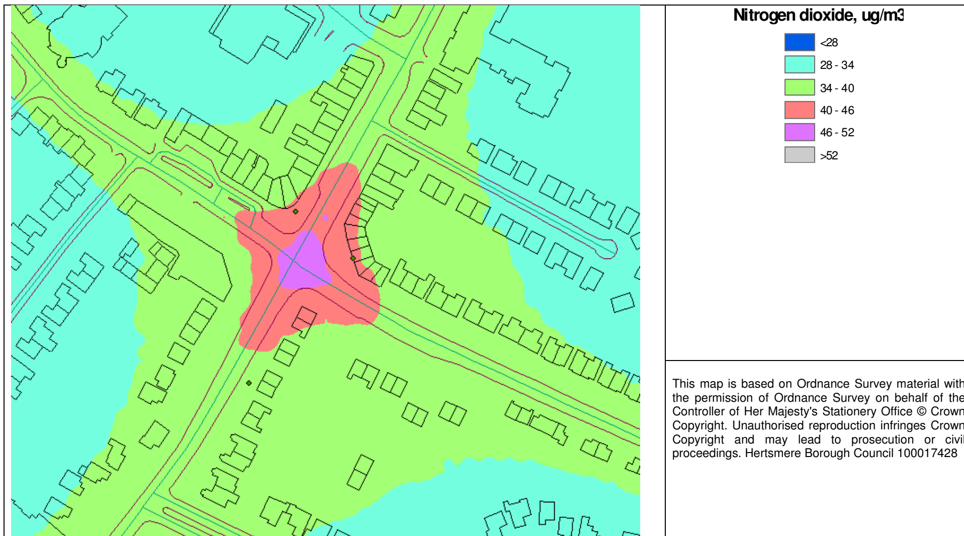
Fig. 3.2: Modelled nitrogen dioxide concentrations, 2010
