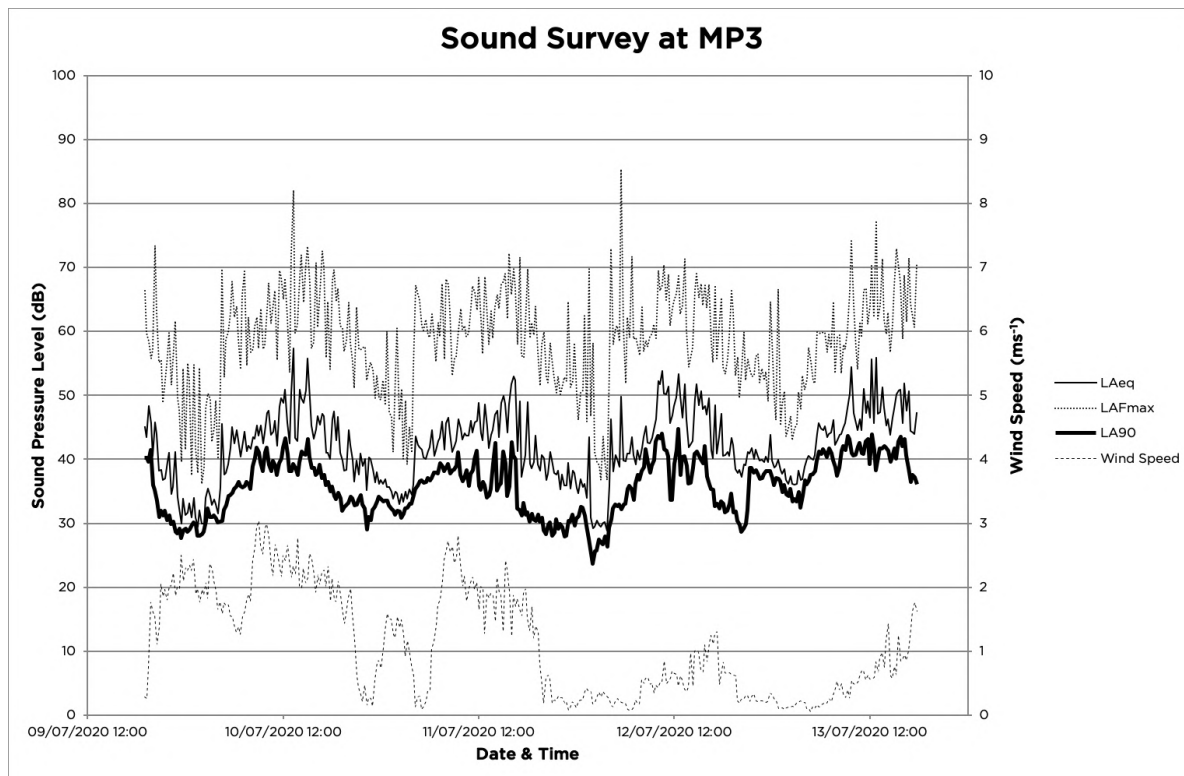
FIGURE 11: MP3 - MEASURED TIME HISTORY
