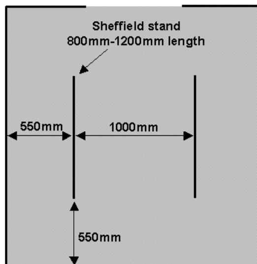
Figure 6: Sheffield stands and indicative cycle store layout (plan view)
