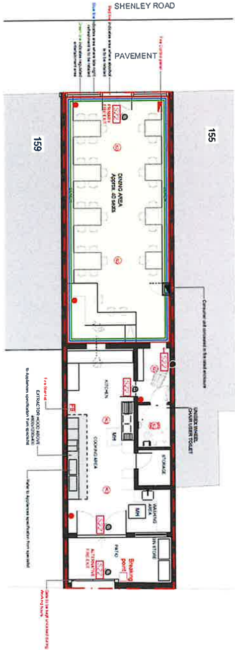
01 Proposed Ground Floor Plan
