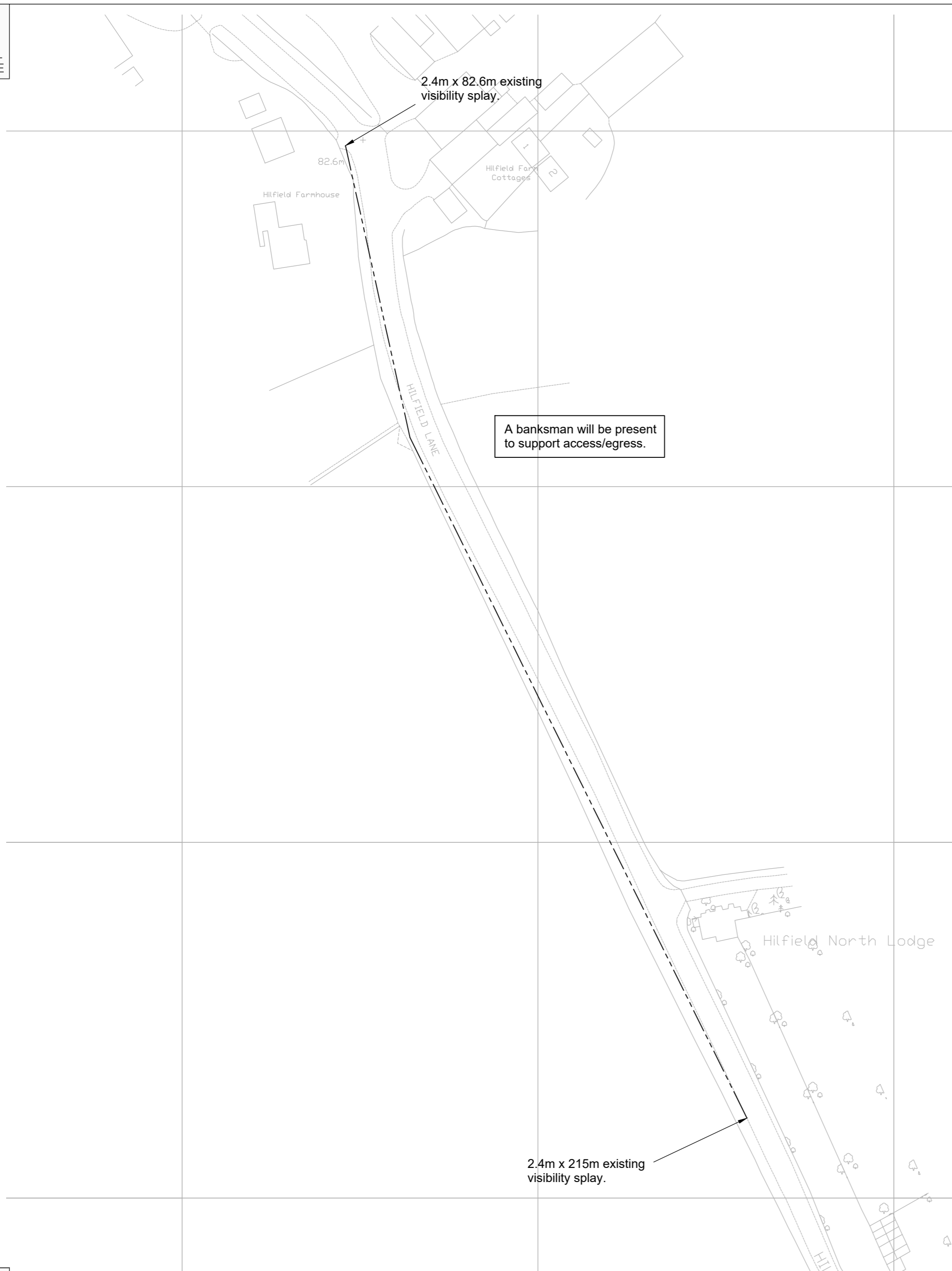
Site Access Arrangement and Visibility Splays
